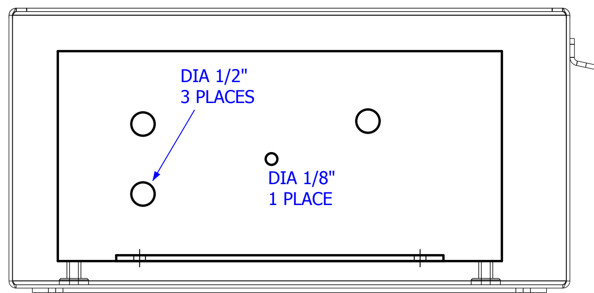
END VIEW
