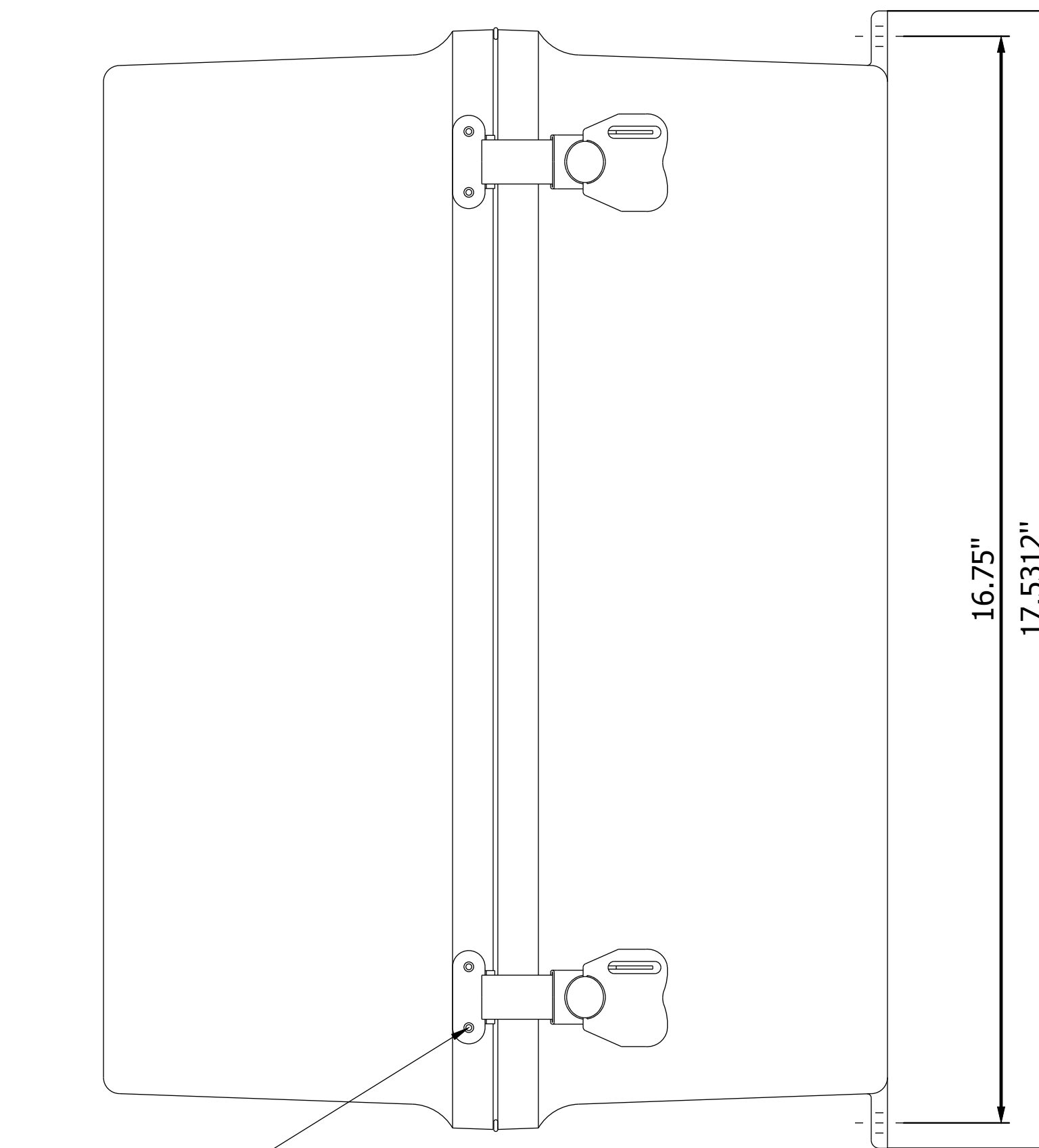
SIDE VIEW (RIGHT)
