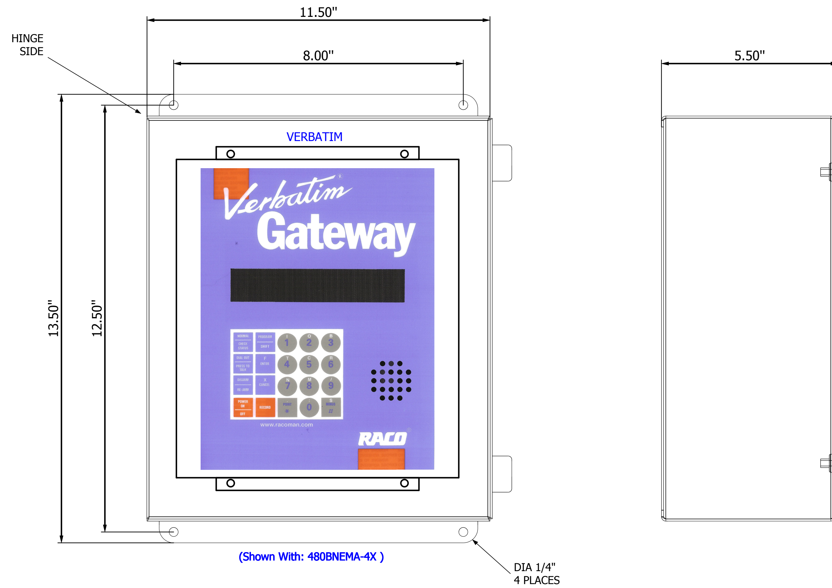
FRONT VIEW
