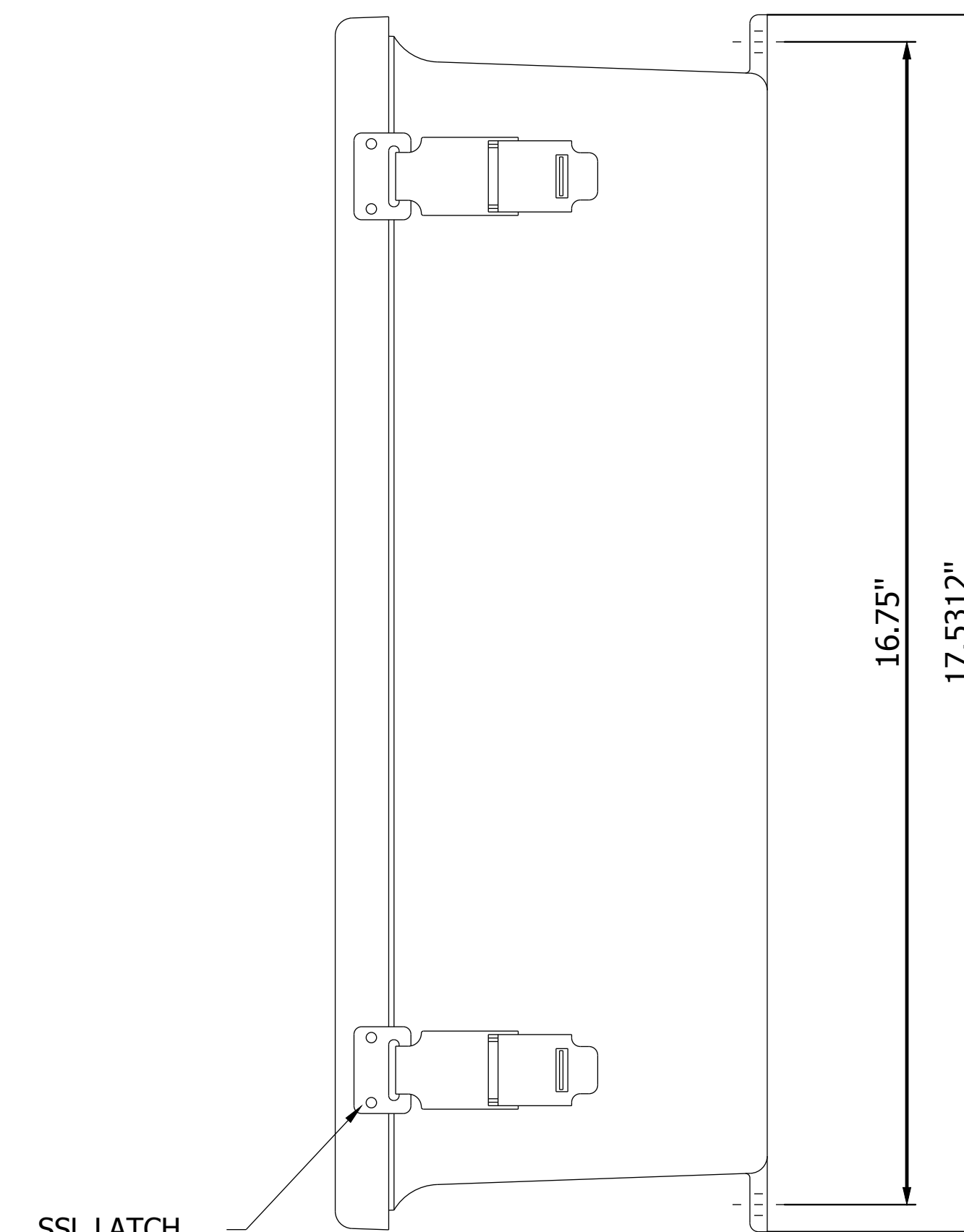
SIDE VIEW
