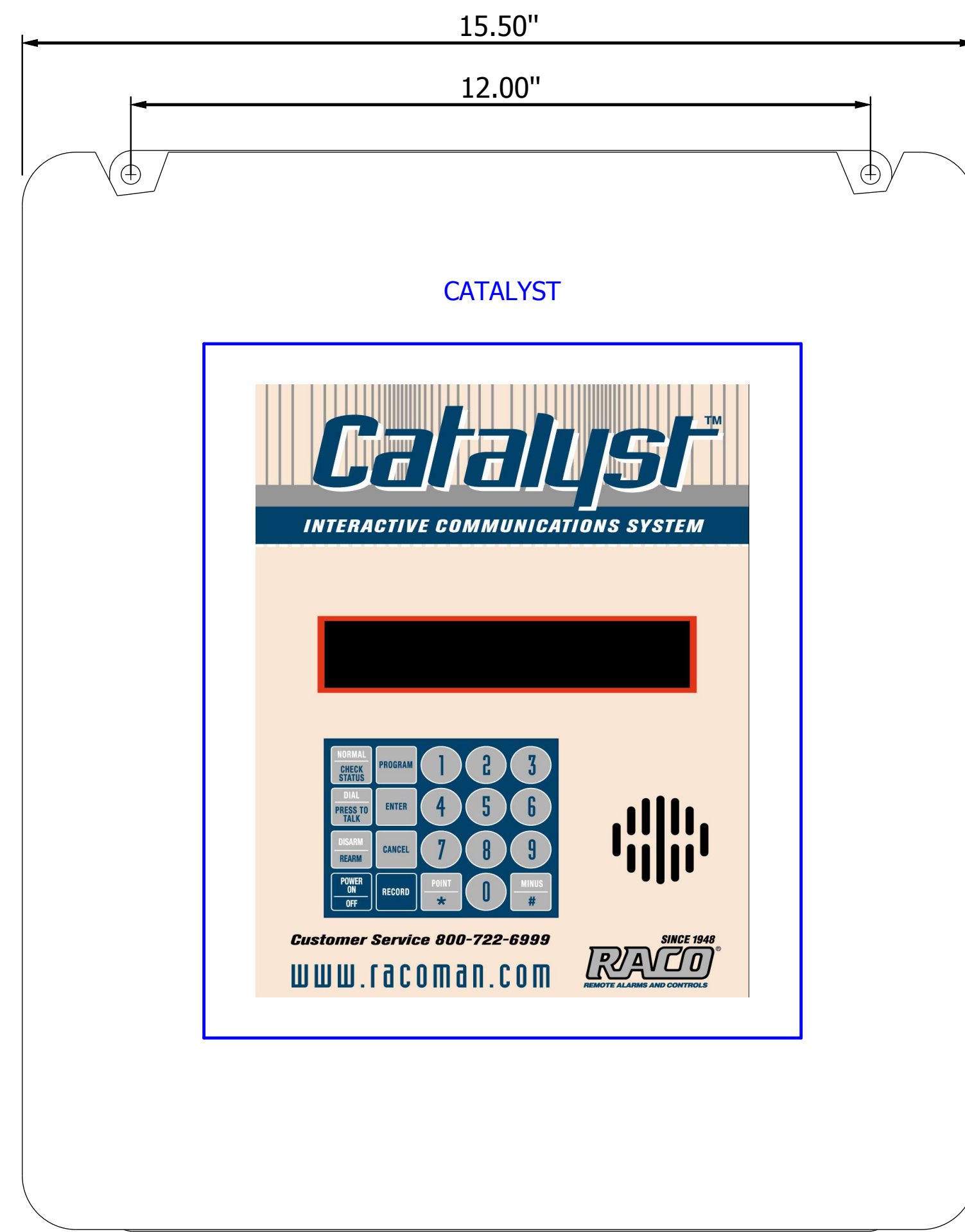
FRONT VIEW
