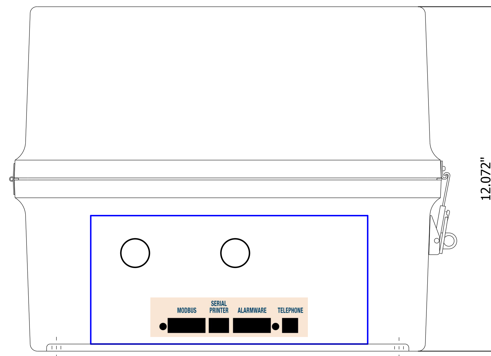
END VIEW
