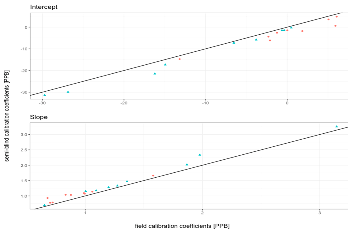
Figure 4. First (red) and last (blue) calibration coefficients for all colocated sites using t_d = 72 h: semibind calibration values \hat{a}_1 (slope) and \hat{a}_0 (intercept) against field calibration values a_1 and a_0 . Line is 1:1 fit.
