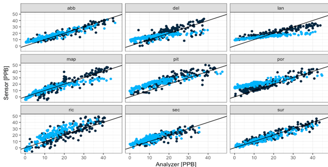
Figure 3. Scatterplots with 1:1 line of the first (dark) and last (light) week of colocated measurements. Data is hourly factory-calibrated sensor data.
