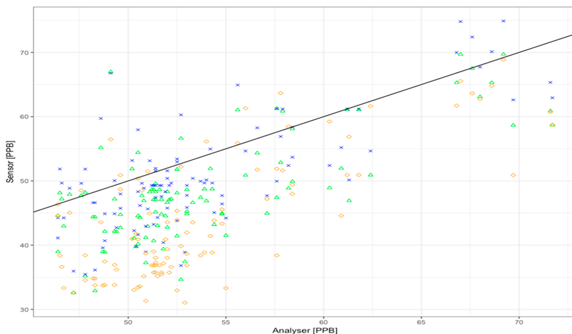
Figure 8. Scatterplot of the 1 min data from Langley location using calibration coefficients derived from the hourly data results ( t_d = 3 days). A random sample of 1000 observations is used for plot clarity. Green triangles = full data set. Blue crosses = left truncation at the mean. Orange diamonds = right truncation at the mean.
