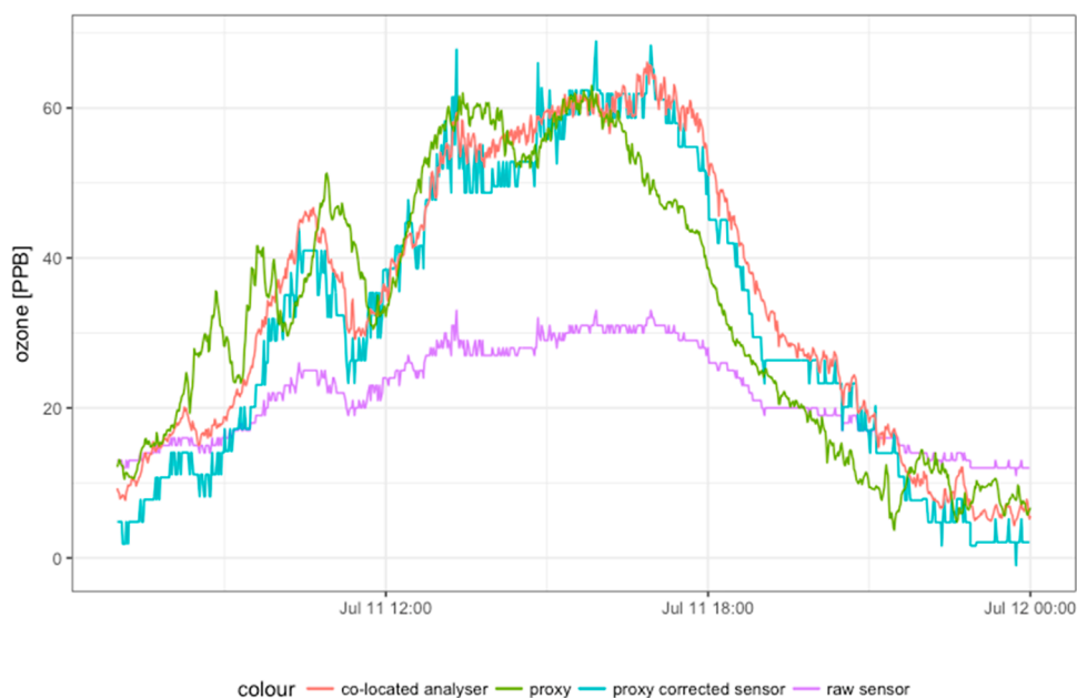
Figure 7. Section of the 1 min data for a collocated site (Langley), comparing the regulatory analyzer and proxy data with the raw and proxy-corrected sensor data.
