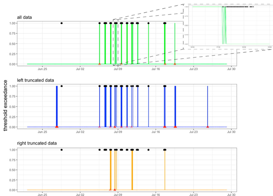
Figure 9. One minute high concentration data as a binary signal for Langlely location using the three different calibration results (all data or a truncation). Colored lines show the corrected sensor results in reporting high concentrations ( >46.2 ppb), where 1 = where a high value has been found, and 0 otherwise. Black points at 1 are false negatives, where a high observation is recorded by the colocated analyzer but not the corrected sensor. Red triangles at 0 are false positives, where a high observation is recorded by the corrected sensor but not the colocated analyzer. The inset shows a close-up where errors may be due to the two instruments recording different air samples causing slight lags.
