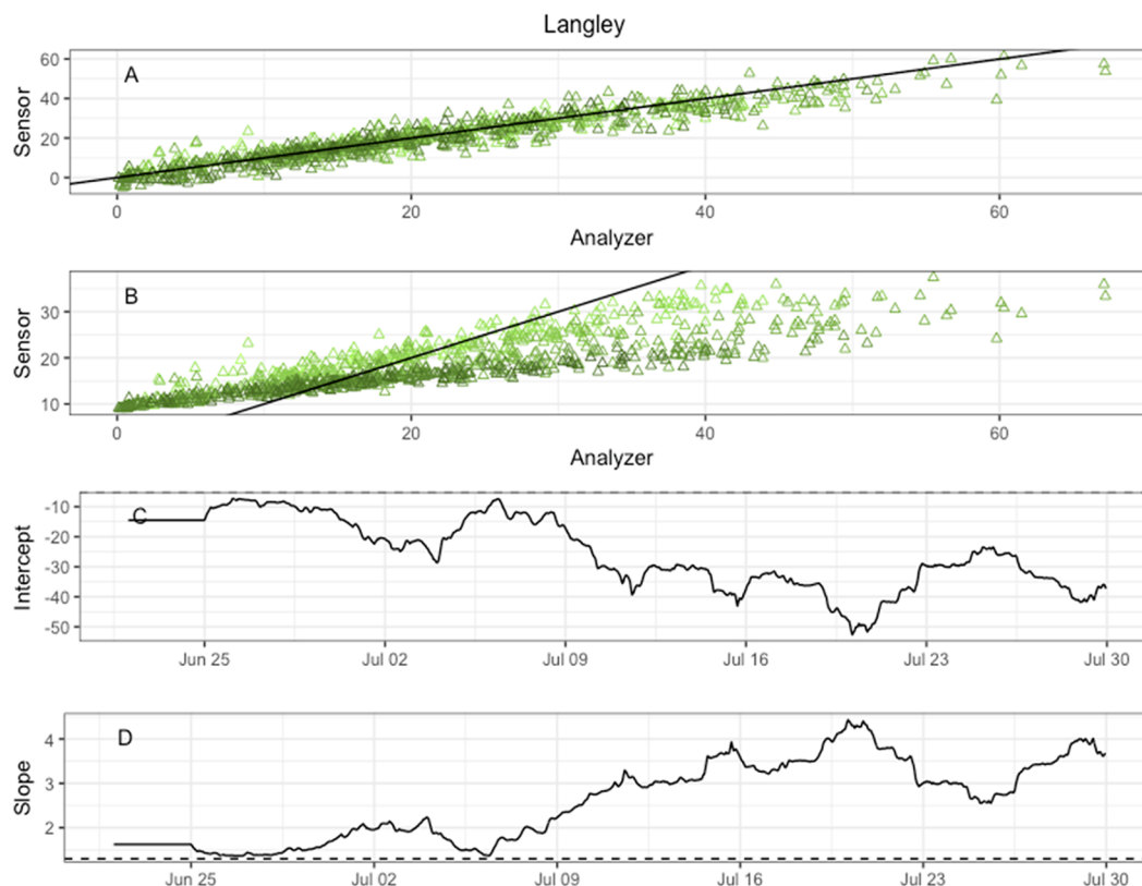
Figure 5. (A) Scatterplot of analyzer and semibind corrected sensor hourly data (earlier weeks = lighter colors and later weeks = darker colors). (B) Similar to (A) using raw sensor data. (C) Stepping intercept estimate, \hat{a}_0 , and (D) stepping slope estimate, \hat{a}_1 , with dashed lines the drift detection thresholds used in ref 22.
