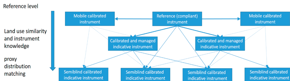
Figure 1. Network architecture for a minimum maintenance, high spatial density air quality measurement network that exploits network cross-correlations. The proxy distribution matching method for “semiblind” calibration is described in the present paper.
