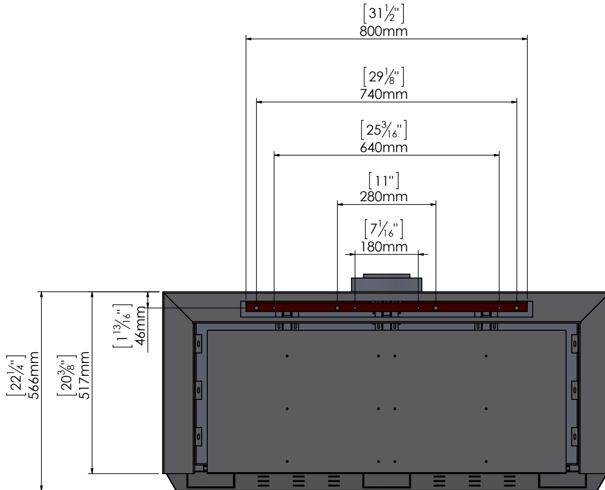
Back View
