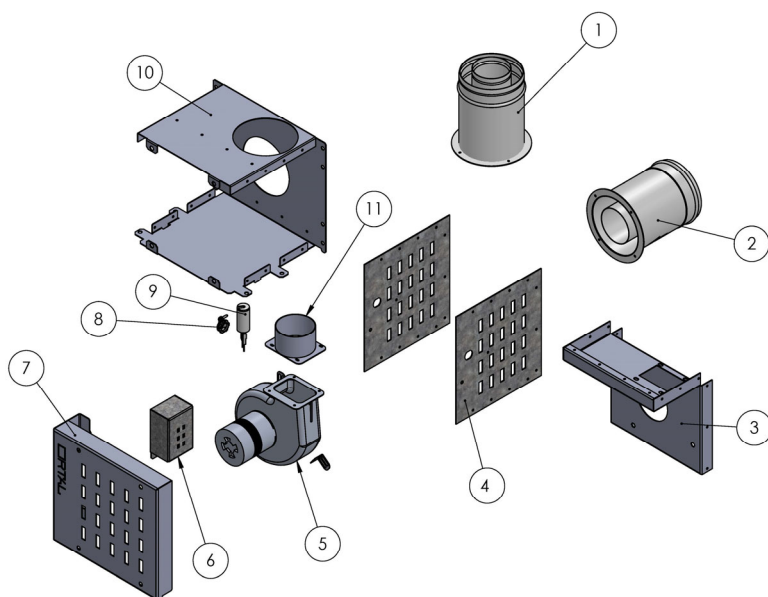
Inline-90 Power Vent Fan Box Components
