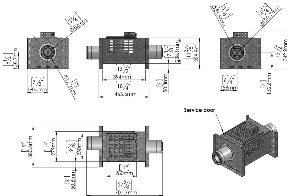
Dimensions for Inline-180 Power Vent
