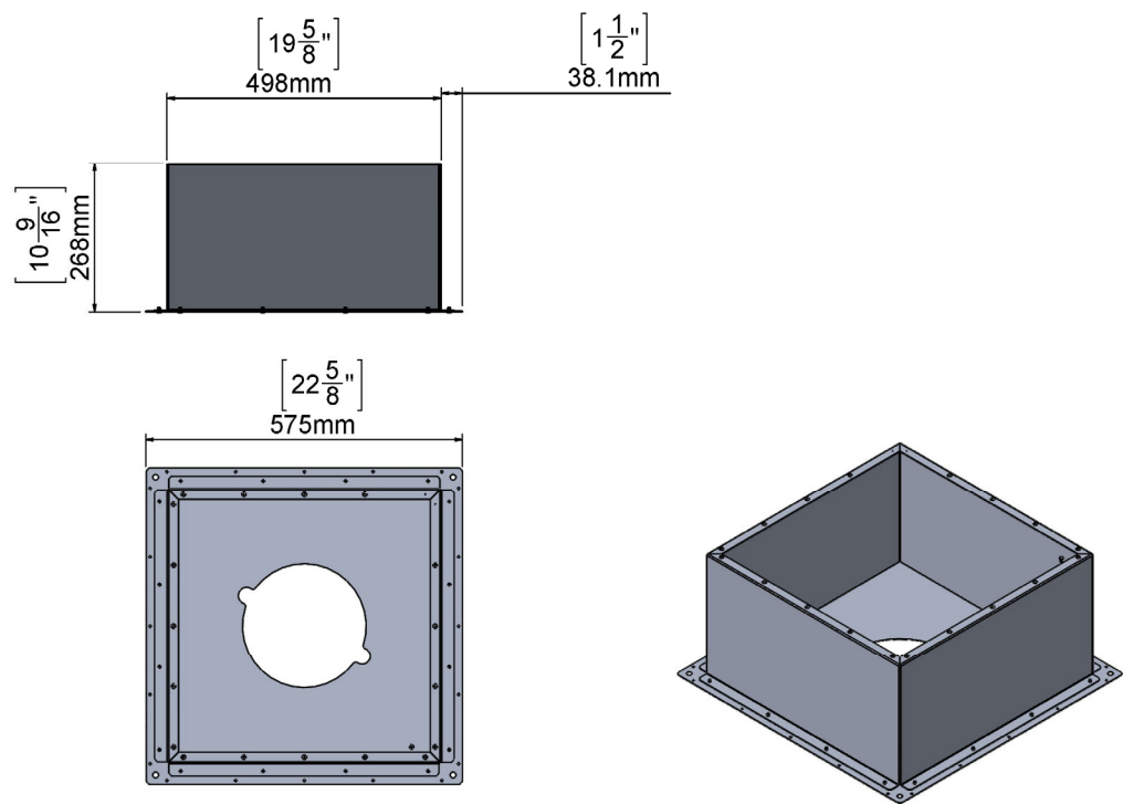
Dimensions for Vertical Termination Power Vent Riser
