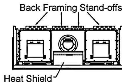
Zero-Clearance Stand-Offs (Top View)
