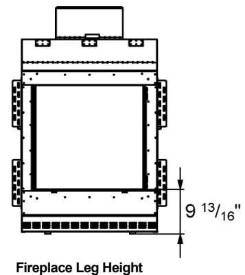
Fireplace Leg Height
