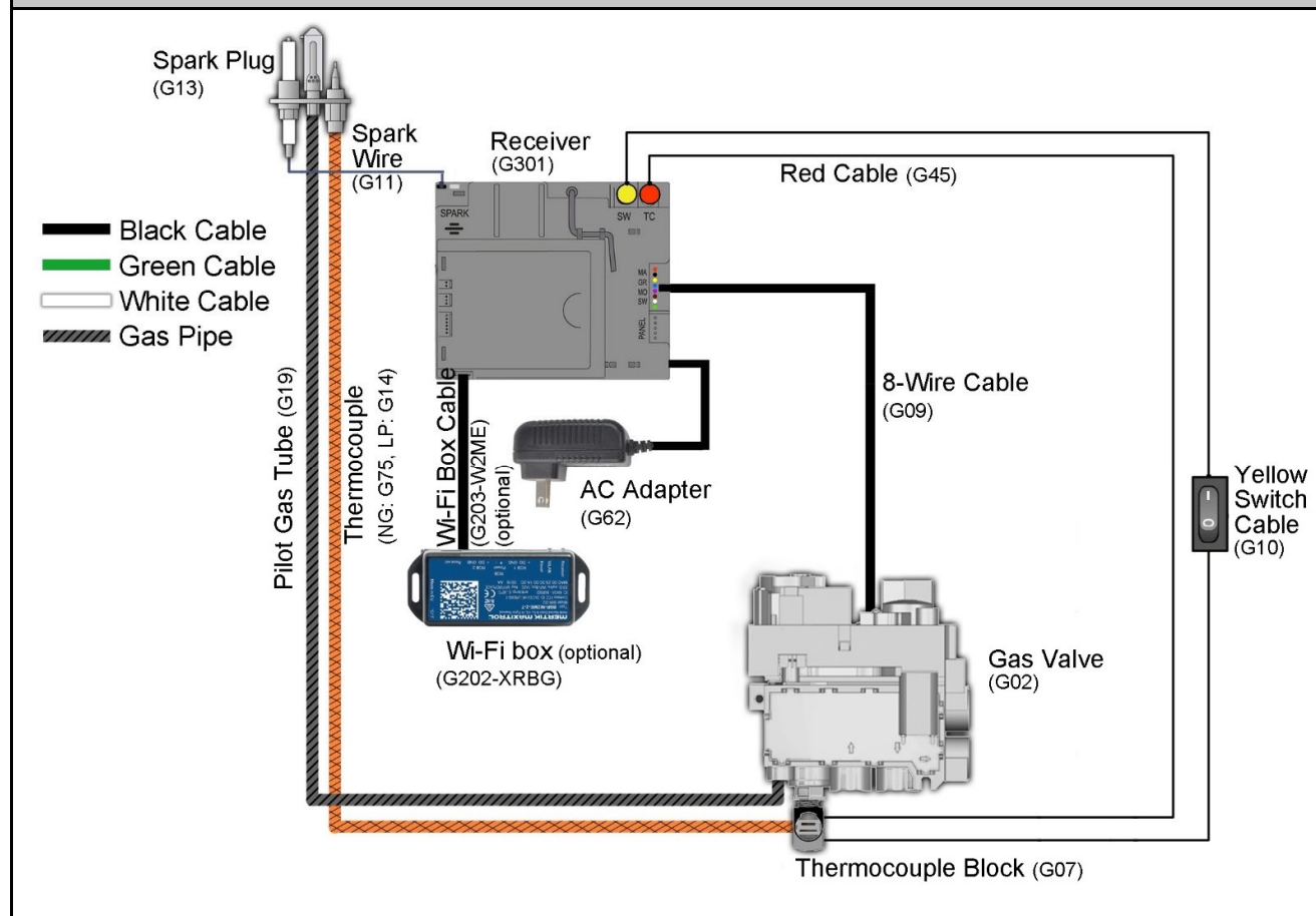
Wiring Diagram: Screen Fireplace
