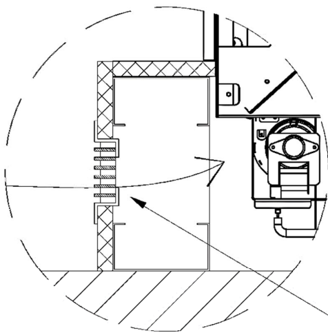
Air Intake as Louvered Grille
