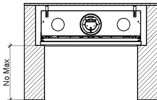
Alcove Side Walls (Top View)
