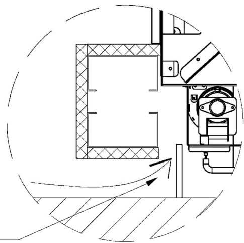
Air Intake as Toe-kick
