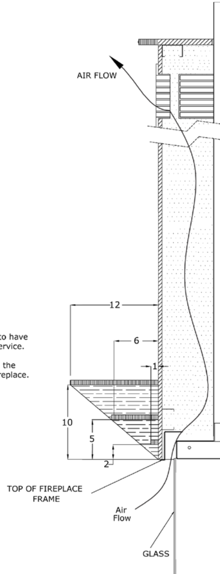
SECTION DETAIL VIEW B-1B
