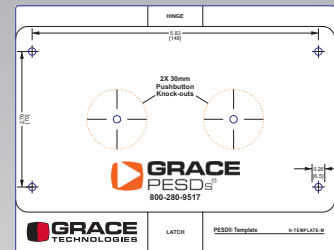
Enclosed Magnetic Template
