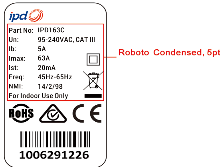
Variant 1 - Ceiec Electric Technology Inc model IPD 163C Electricity Meter
