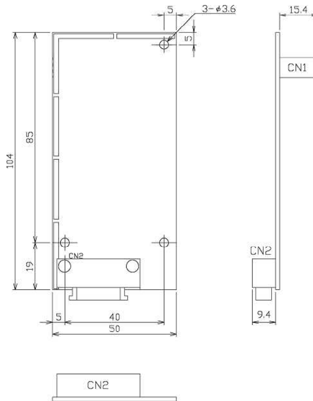
Figure 1.2-1 External Appearance
