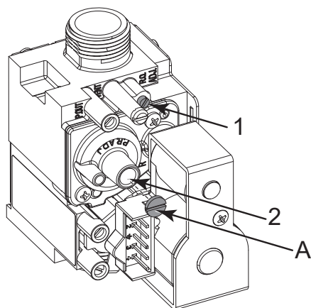
Figura 6.5 Valvola gas
