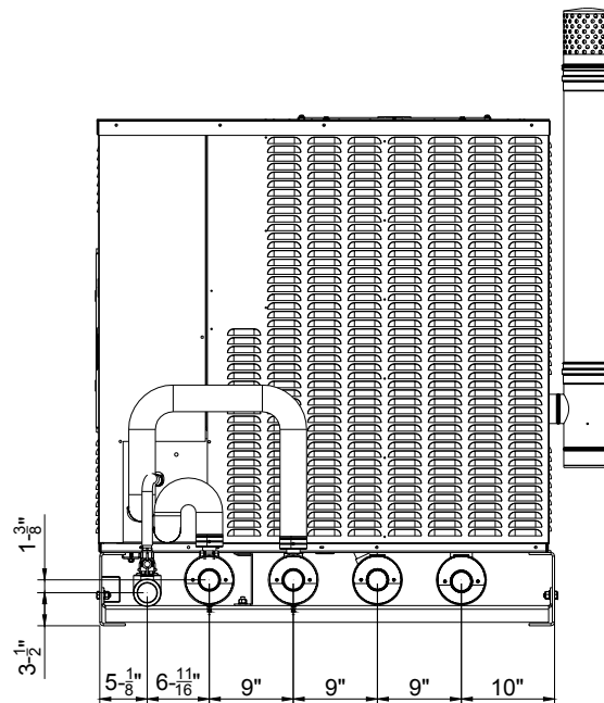
Figure 1 - RTYF anti-vibration supports positioning dimensions and piping specifications; dimensions in inches unless otherwise specified.
