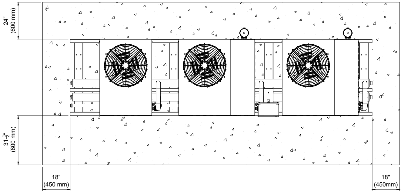
Figure 3 - Minimum clearances from obstacles, walls and combustibles surfaces.
