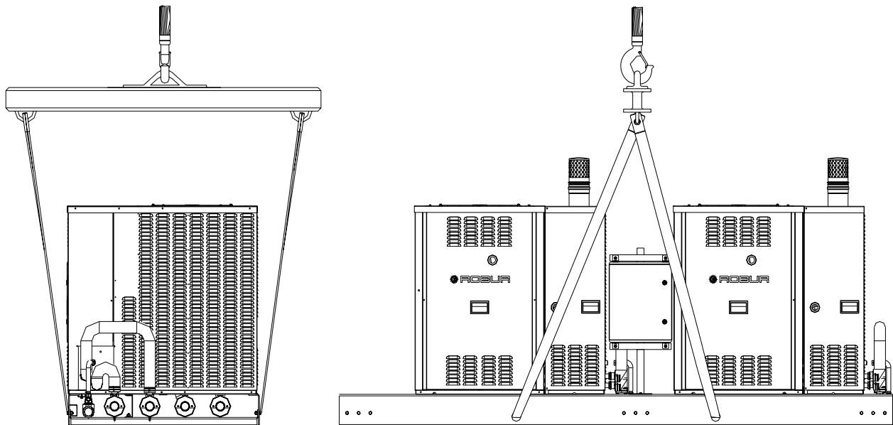
Figure 2 - Lifting the appliance. Example for a RTYF 120-238.
