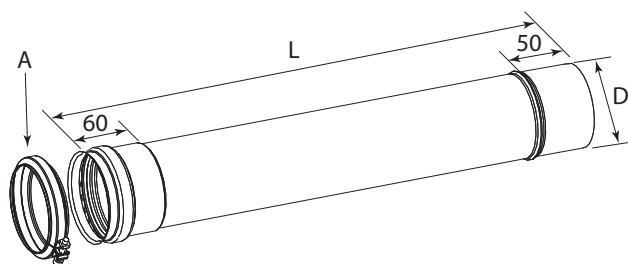
Figure 1.1 Pipe
