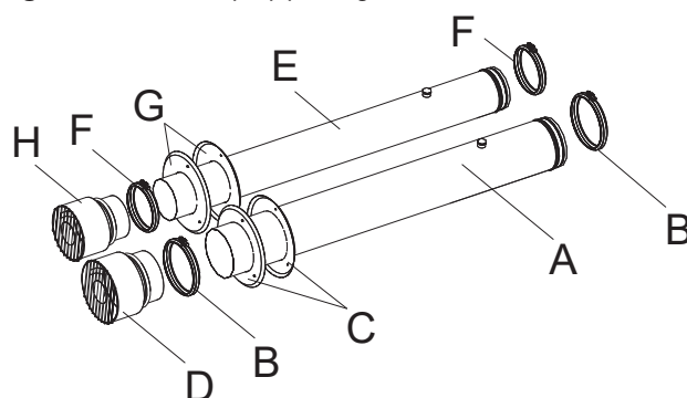
Figure 3.2 OSCR004 split pipe flue gas exhaust
