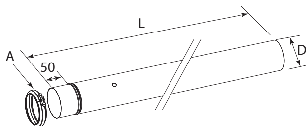
Figure 1.2 Pipe with flue gas analysis socket
