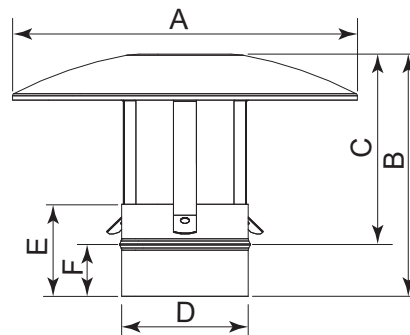
Figure 6.1 Roof terminal
