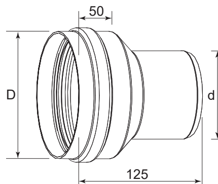
Figure 1.3 Adapter for exhaust/air pipes
