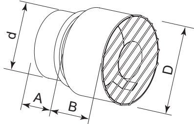
Figure 6.2 Wall terminal
