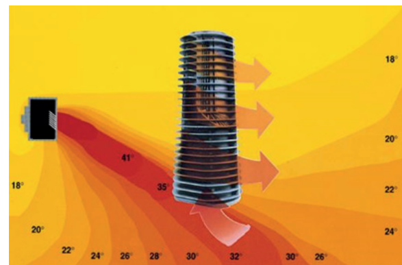
Figure 2.6 Robur heat exchanger ground effect
