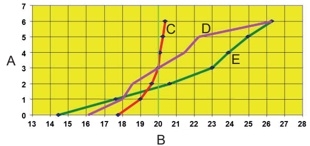
Figure 3.4 Heating appliances stratification diagram
