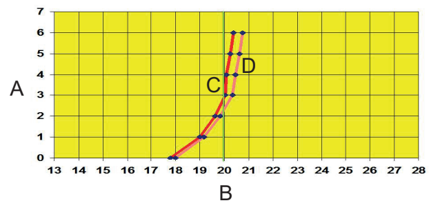
Figure 3.5 Stratification of Robur gas unit heaters with and without destratifiers
