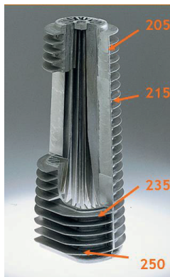
Figure 2.4 Robur heat exchanger temperature
