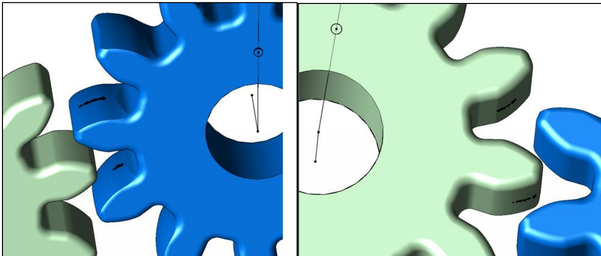
Figure 10. Angle Backlash Drive Flank Contact
