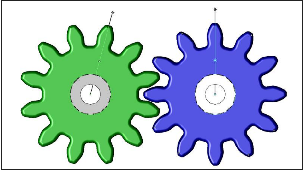
Figure 2. A 15° rotated position of the green Drive Gear with the Multi Tooth, Rotational Contacts for Axial Backlash and F_i'' .
