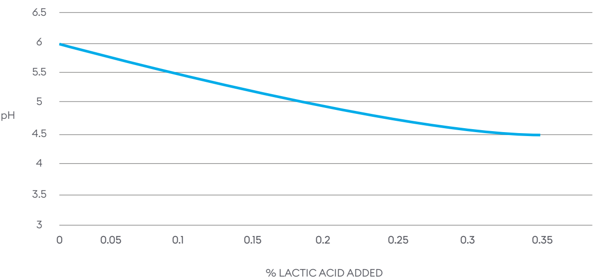
Fig.2: Graph to show Syndopal pH adjustment from additional lactic acid solution.
