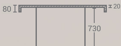
CROSS-SECTION VIEW
